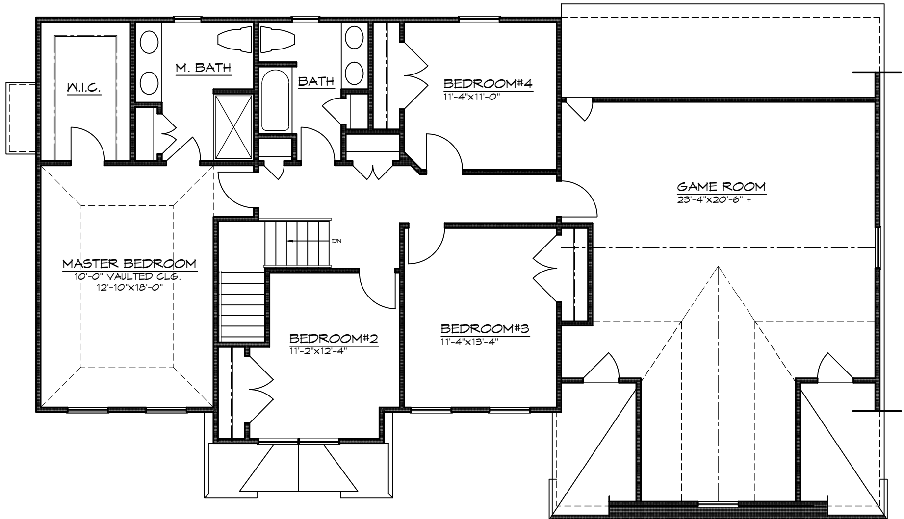
SECOND FLOOR PLAN SECOND FLOOR - 1,713 S.F.
